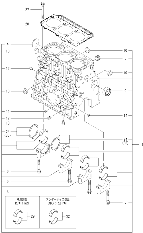
0CW10-M47400 3TNV84T-BKSA Fig.1. CYLINDER BLOCK
