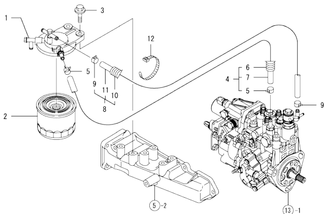
Fig.16. FUEL LINE
