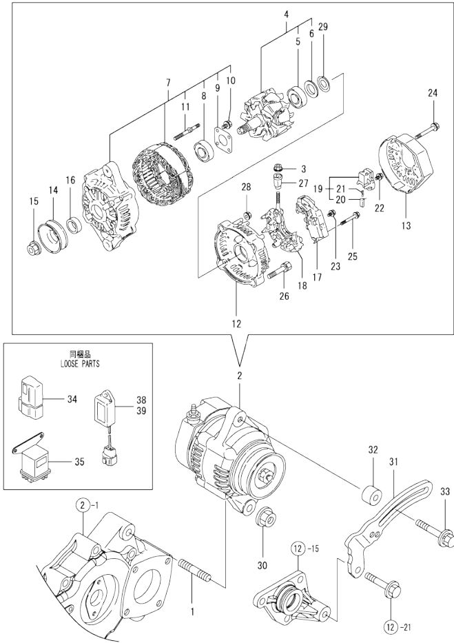
0CW10-M47400 3TNV84T-BKSA Fig.18. GENERATOR
